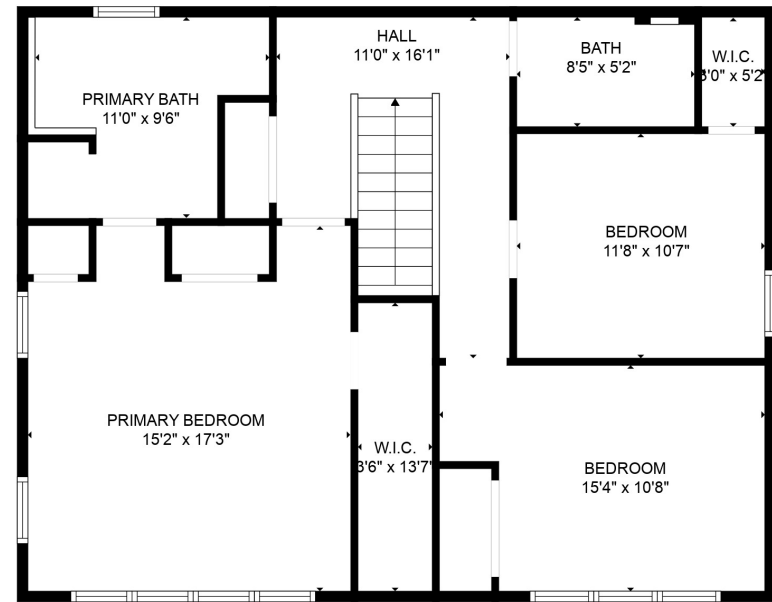
FLOOR 3
