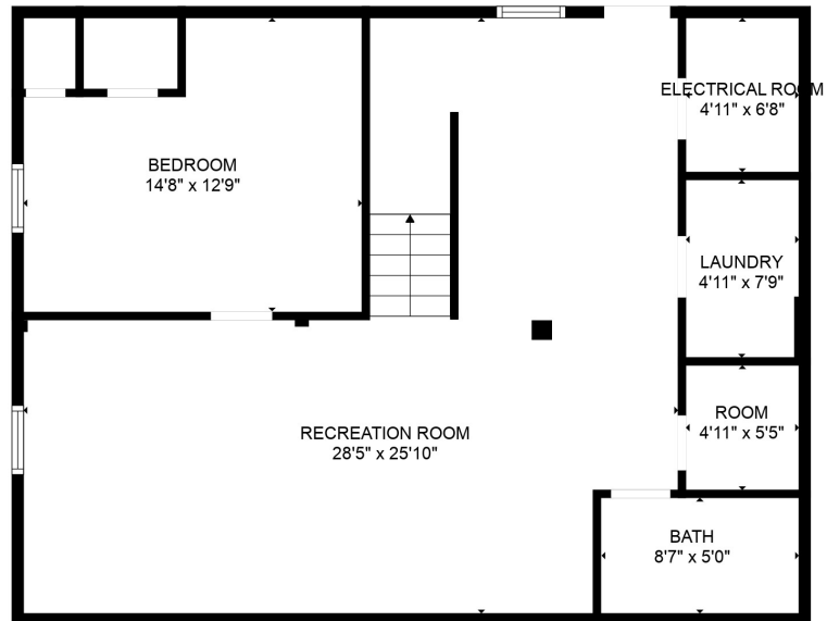
FLOOR 2
