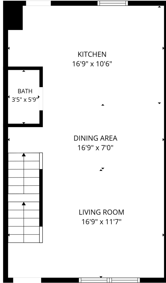
1st floor
